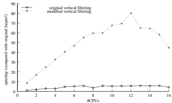
Figure 11. Parallel Runtime Analysis of Jasper (16384 Kpixel image, SGI): Speedup for original and improved filtering with respect to the original Jasper runtime
