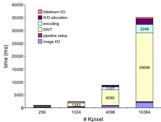
Figure 6. Parallel Runtime Analysis of JJ2000 on SMP (four processor Compaq, Intel Pentium II Xenon, 500 MHz)
