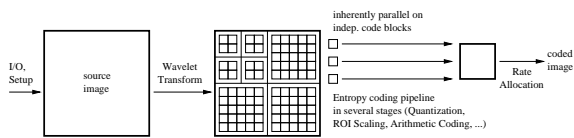
Figure 1. JPEG2000 coding pipeline
