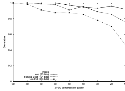
(a) JPEG
