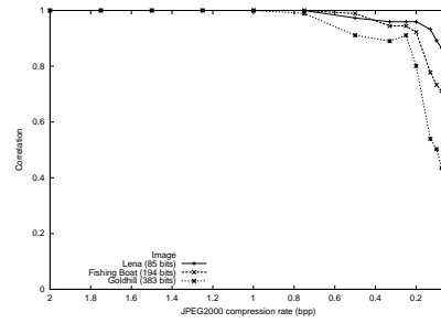
(b) JPEG2000
