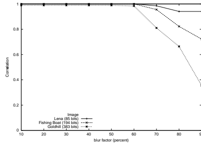
(c) blur
