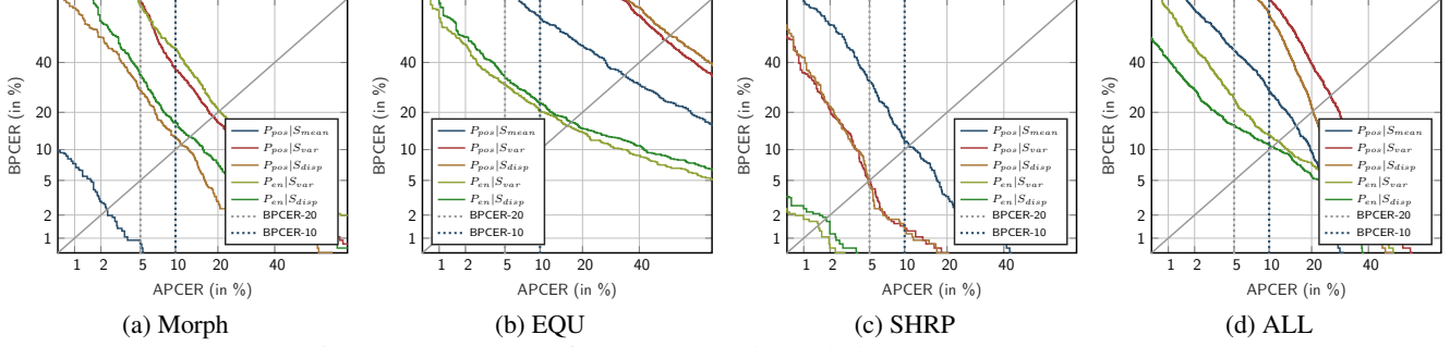
Figure 7: DET curves for PRNU-based morph detectors ( 10 \times 10 cells).
