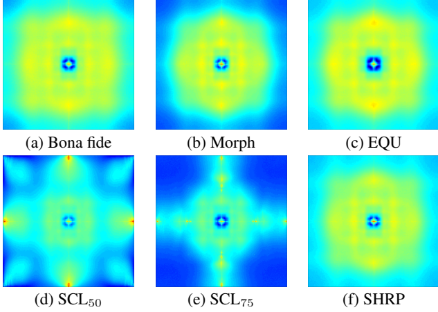
Figure 3: Averaged PRNU DFT magnitude spectra of bona fide images (a), morphed images (b) and post-processed morphed images (c to f).
