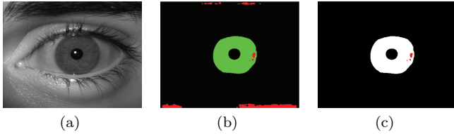
Fig. 10: Sample iris image with P0 gaze-angle (10a) and its corresponding segmentation (green area) and error mask (red area) before (10b), and after correction (10c), using the network trained on P0 images
