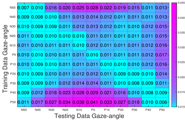
Fig. 12: Segmentation performance on the different gaze-angle groups under the improved-homogeneous approach as average nice1 error
