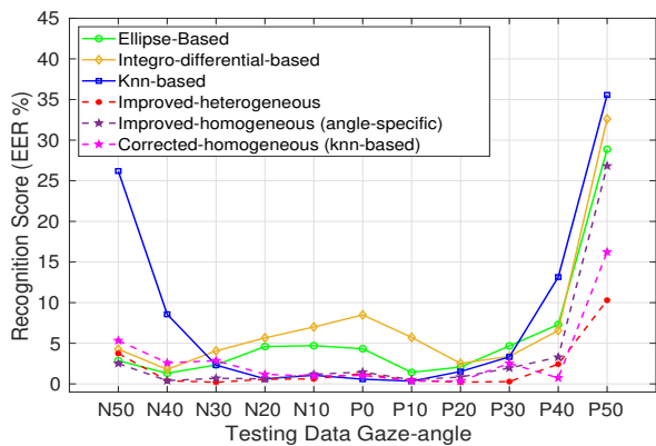
Fig. 25: Recognition performance on the different gaze-angle groups under the corrected-frontal approach, using the different correction algorithms, in terms of EER error
