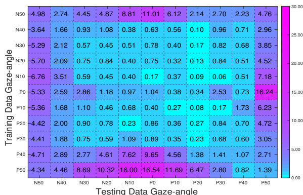
Fig. 18: Recognition performance on the different gaze-angle groups under the corrected-homogeneous approach, using the KNN-based algorithm, in terms of ER error
