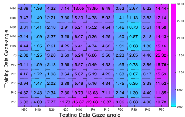
Fig. 19: Recognition performance on the different gaze-angle groups under the corrected-homogeneous approach, using the Integrodifferential-based algorithm, in terms of ER error
