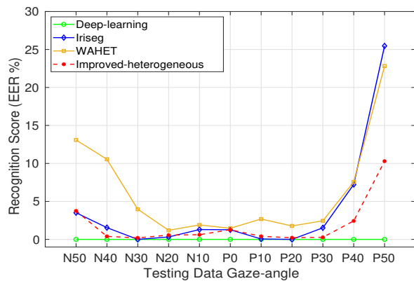
Fig. 26: Recognition performance on the different gaze-angle groups using the different recognition algorithms, in terms of EER error
