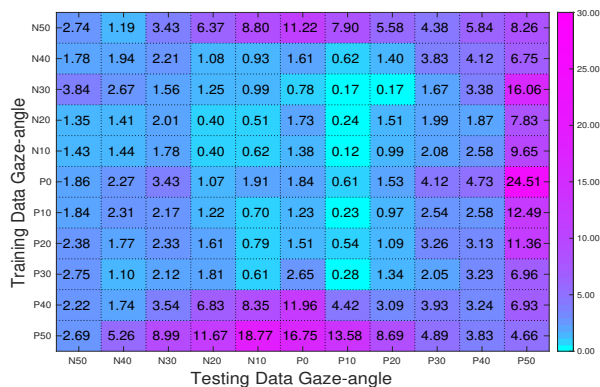
Fig. 21: Recognition performance on the different gaze-angle groups under the corrected-homogeneous approach, using the Ellipse-based algorithm, in terms of EER error
