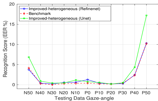
Fig. 16: Recognition performance benchmark and the corresponding experimental results on the different gaze-angle groups under the improved-heterogeneous approach using different CNNs, in terms of EER error
