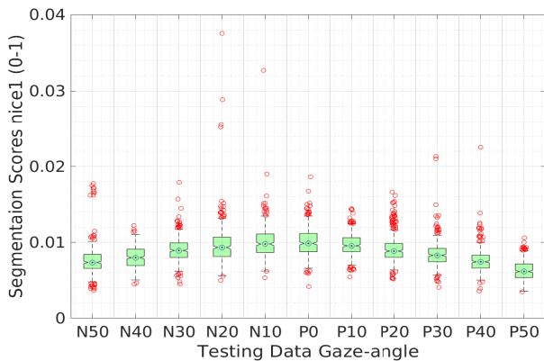
Fig. 14: Segmentation performance on the different gaze-angle groups under the improved-heterogeneous approach as average nice1 error
