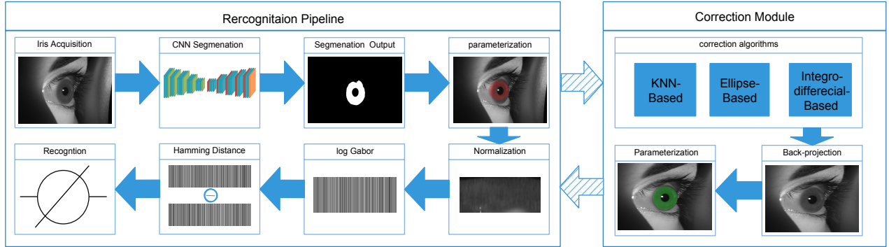
Fig. 9: Recognition pipeline and the correction module
