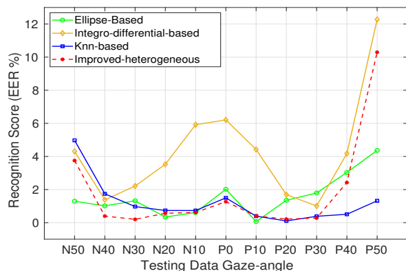
Fig. 23: Recognition performance on the different gaze-angle groups under the corrected-heterogeneous approach, using the different correction algorithms, in terms of EER error
