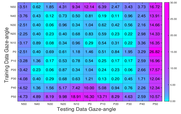
Fig. 13: Recognition performance on the different gaze-angle groups under the improved-homogeneous approach in terms of EER error
